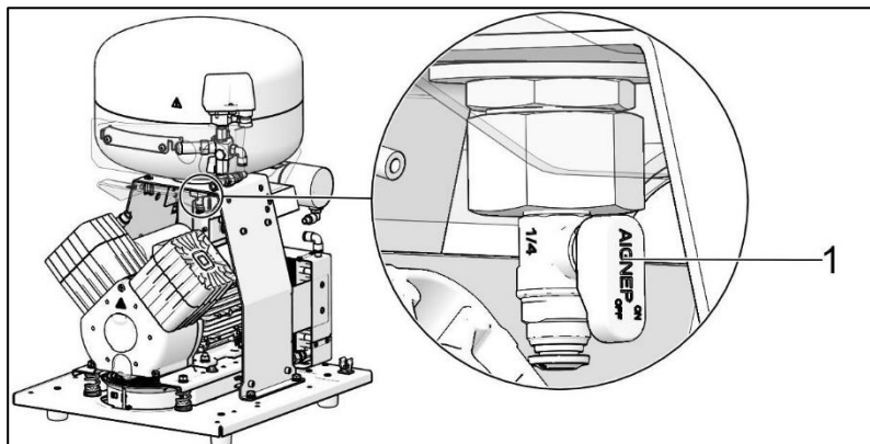
Fig. 6: Condensate drain
