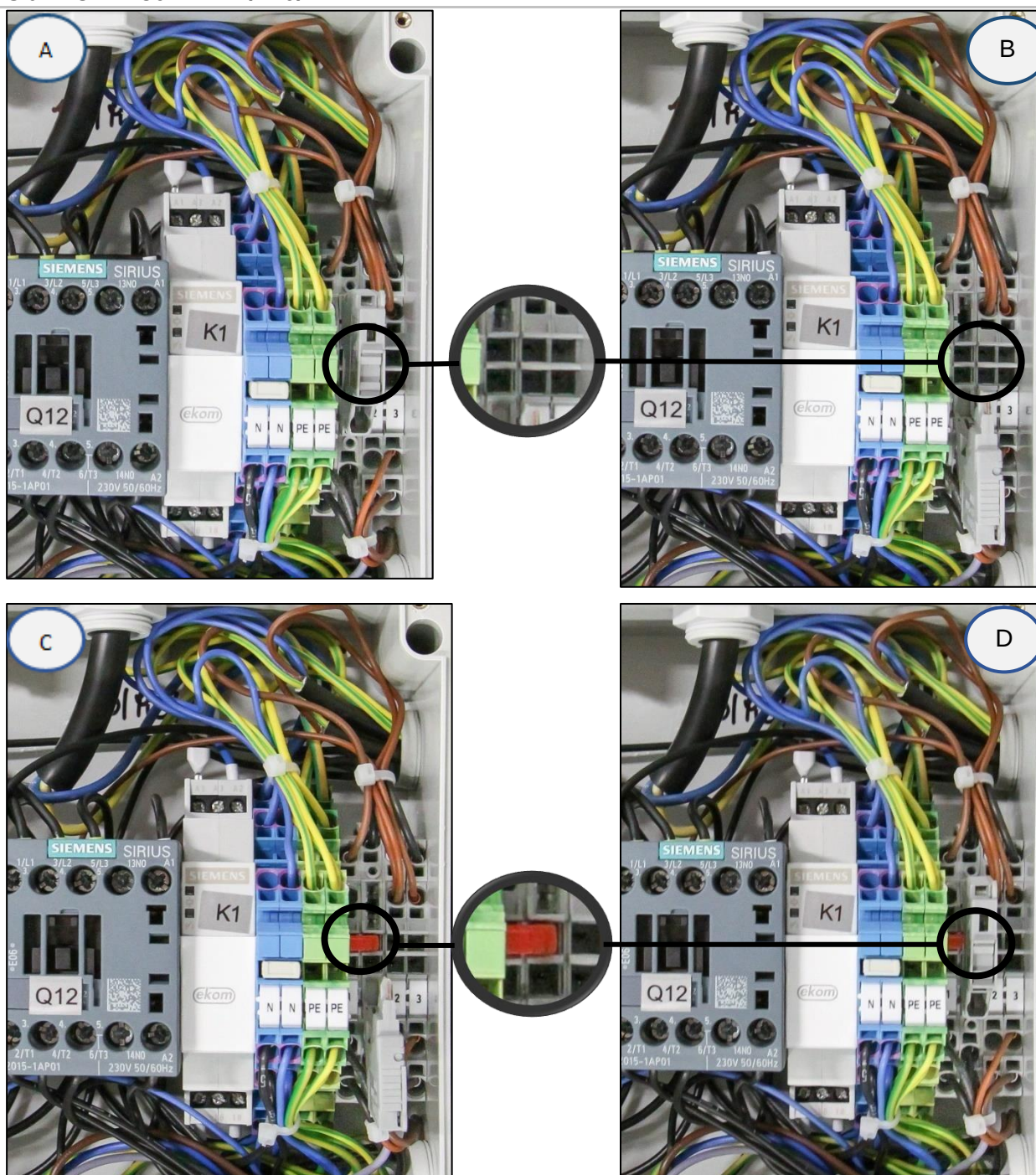
Obr. 28: DK50 2x4VR/110/M
