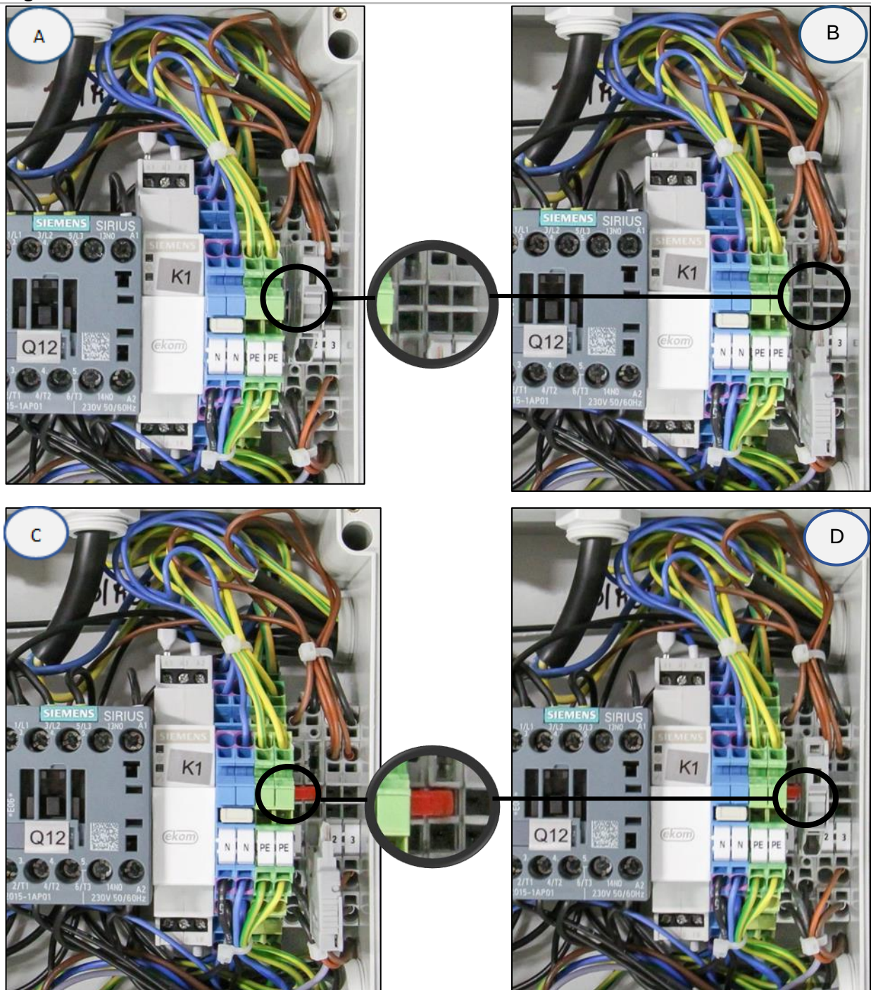
Fig. 28: DK50 2x4VR/110/M
